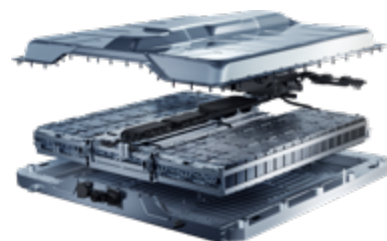
Pack batterie DHB (Dedicated Hybrid Battery)
